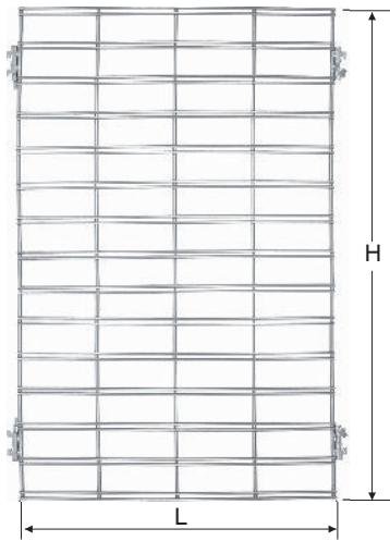
Mesh Panel
