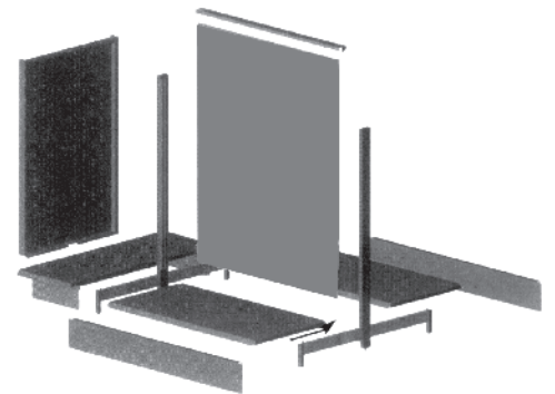
Typical Construction
